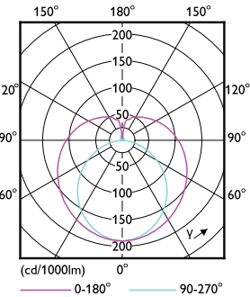
Light Distribution Diagram - 43T8/COR/96-5CCT/MF52LS/G/FA8-R17D 10/1
