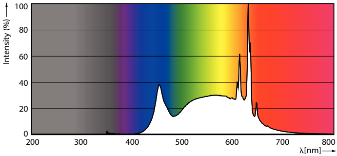
Spectral Power Distribution Colour - 14A19/COR/940/FR/P/E26/DIM/T20 6/1CT
