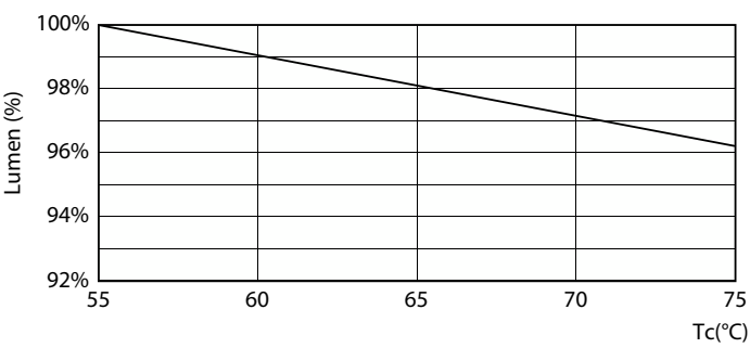
Lumen Maintenance Diagram - 10.5T8/COR/36-5CCT/FF15/G/DIM 25/1
