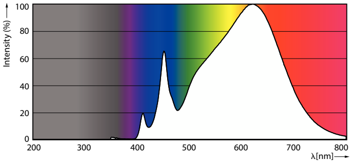
Spectral Power Distribution Colour - 14PAR38/EXPERTCOLOR RETAIL/ F25/930/P/D/B
