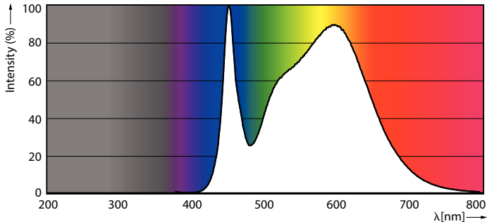
Spectral Power Distribution Colour - 115CC/LED/840/LS EX39 G2 BB 277-480V 3/1
