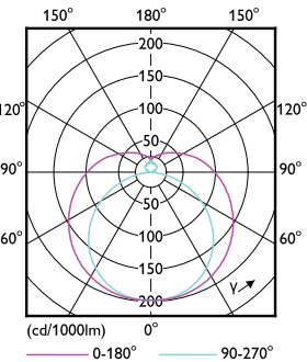
Light Distribution Diagram - 24T5HO/COR/46-840/IF35/G/DIM 25/1
