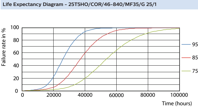
Life Expectancy Diagram - 25T5HO/COR/46-840/MF35/G 25/1
