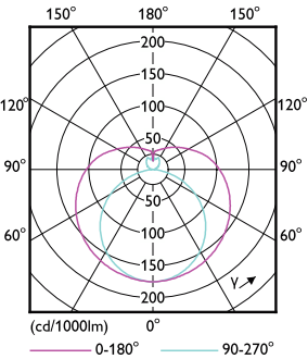
Light Distribution Diagram - 25T5HO/COR/46-835/MF33/G 25/1
