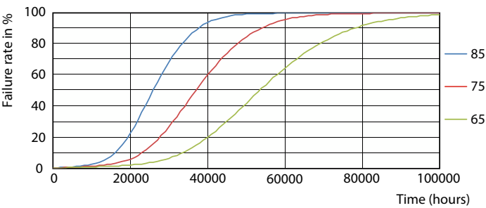
Life Expectancy Diagram - 17PL-L/COR/22-835/MF22/G/4P 10/1
