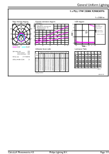
General uniform lighting - 17PL-L/COR/22-835/MF22/G/4P 10/1
