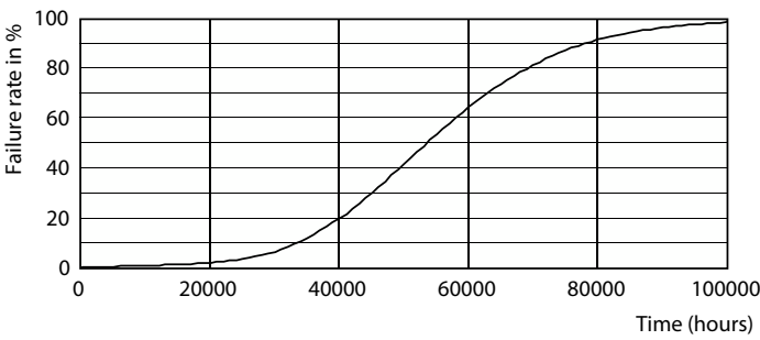
Life Expectancy Diagram - 17PL-L/COR/22-835/MF22/G/4P 10/1
