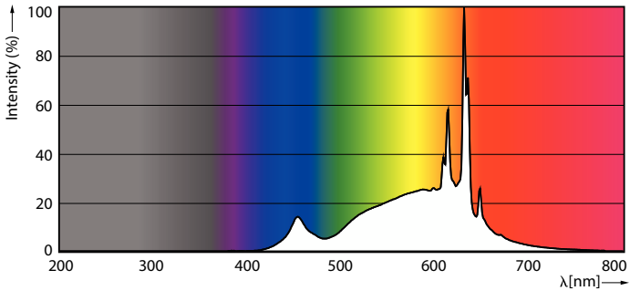
Spectral Power Distribution Colour - 12.2A19/PER/927/P/E26/DIM 6/1FB T20
