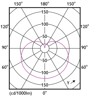
Light Distribution Diagram - 12.2A19/PER/927/P/E26/DIM 6/1FB T20
