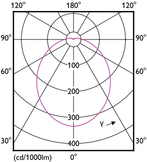
Light Distribution Diagram - 5R20/PER/927/P/E26/DIM 6/1FB T20
