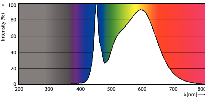
Spectral Power Distribution Colour - 15.5T8/MAS/48-835/IF24/P/DIM 25/1
