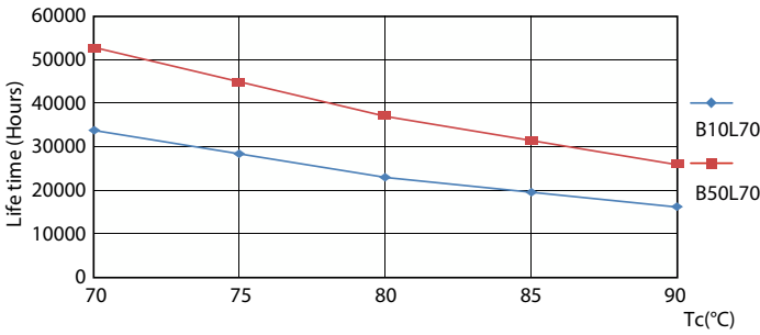
Life Expectancy Diagram - 14T5HE/46-850/IF21/G/DIM 10/1
