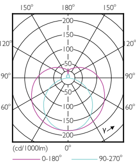
Light Distribution Diagram - 11T5HE/34-850/IF15/G/DIM 10/1
