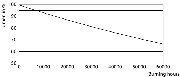
Lumen Maintenance Diagram - 11T5HE/34-850/IF15/G/DIM 10/1
