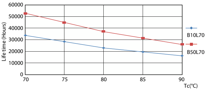
Life Expectancy Diagram - 11T5HE/34-850/IF15/G/DIM 10/1
