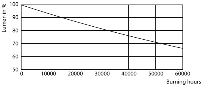
Lumen Maintenance Diagram - 8T5HE/22-840/IF10/G/DIM 10/1
