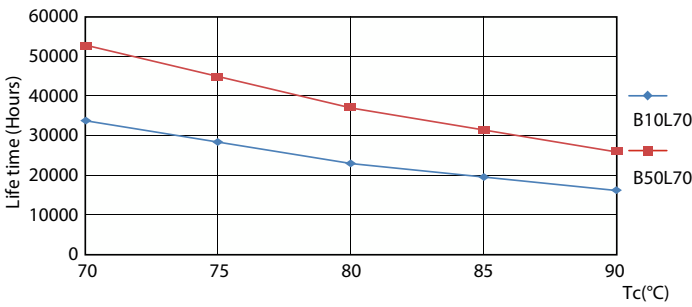
Life Expectancy Diagram - 8T5HE/22-840/IF10/G/DIM 10/1
