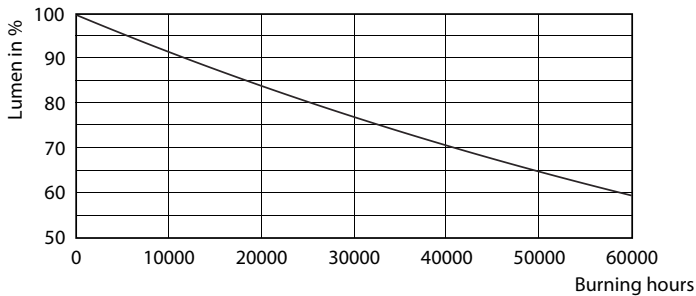
Lumen Maintenance Diagram - 12PAR30L/EXPERTCOLOR/F40/927/DIM
