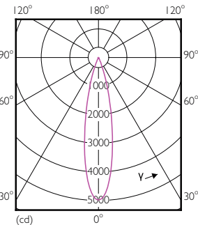
Light Distribution Diagram - 12PAR30L/EXPERTCOLOR/F40/927/DIM
