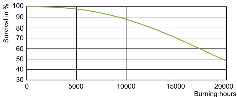
Life Expectancy Diagram - MHC50/U/MP/3K ELITE
